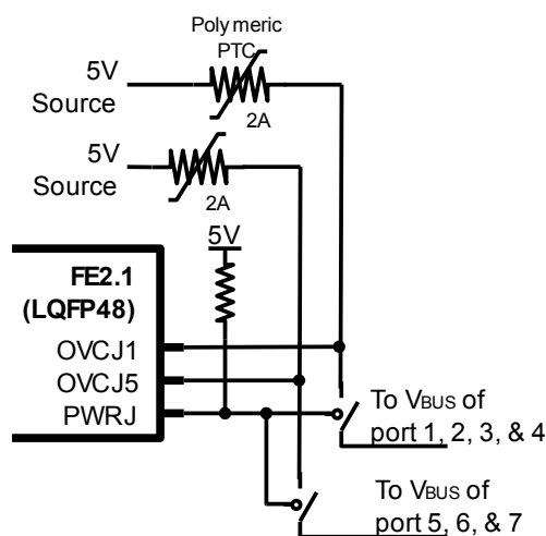
Fig. 8: LQFP-48 Power Control Example
